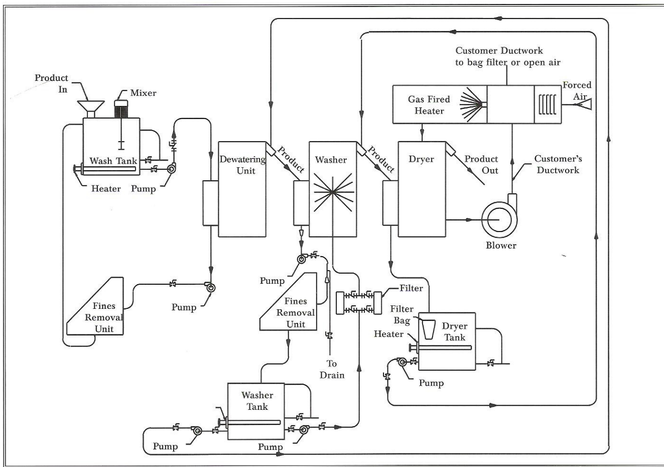
Schematic Flow Diagram of a typical Recycle System
